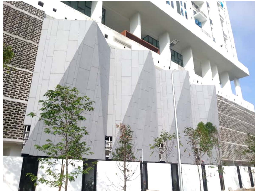
Design & Install façade framing with combination of mild steel Hollow Frame ; light gauge Top Hat profiles & Cladded with Compressed fiber cement sheet
