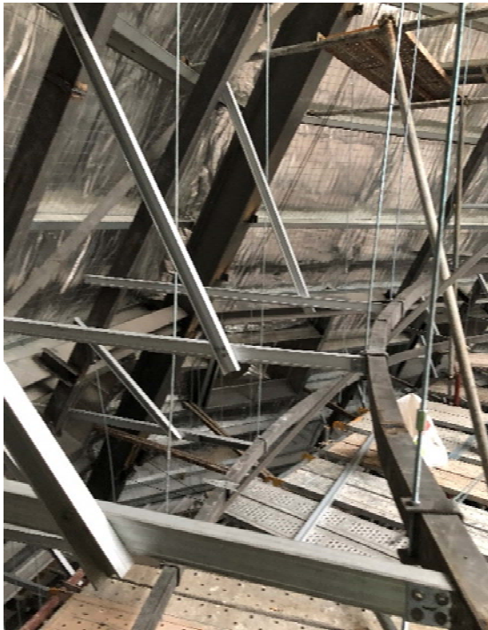
Pre Curved RHS ring beam & Pre Curved furring channel to form Dome ceiling with 2 layer plasterboard
