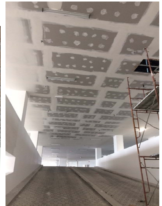
Ceiling frame with plasterboard installed
